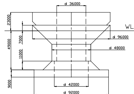
Fig.1 Floating monocon moored by sloped tensioned legs [1]
