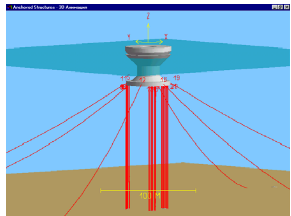
Figure 4. TLP operational intact position under ice influence
